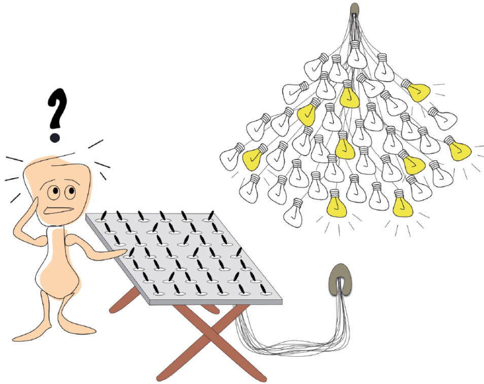
Fig. 1. How do animals develop sensorimotor maps linking motoneurons and muscles? Initially, the mapping relations are unknown, metaphorically illustrated here by a bank of switches (neurons) connected in unknown ways to a cluster of light bulbs (muscles). Faced with this confusion, the guy at the switchboard would be wise to throw each switch one at a time and tally the lights that turn on. Analogously, animals may use discrete twitches during sleep to establish, refine, maintain, and repair sensorimotor circuits throughout the nervous system. Reprinted from “Twitching in Sensorimotor Development From Sleeping Rats to Robots,” by M. S. Blumberg, H. G. Marques, and F. Iida, 2013, Current Biology , 23, p. R533. Copyright 2013 by Elsevier. Adapted with permission.
